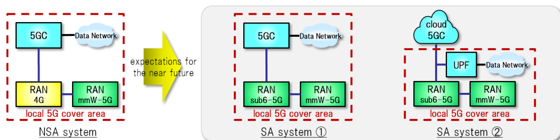
Fig. 7.3-3 System configuration example for local 5G millimeter wave
