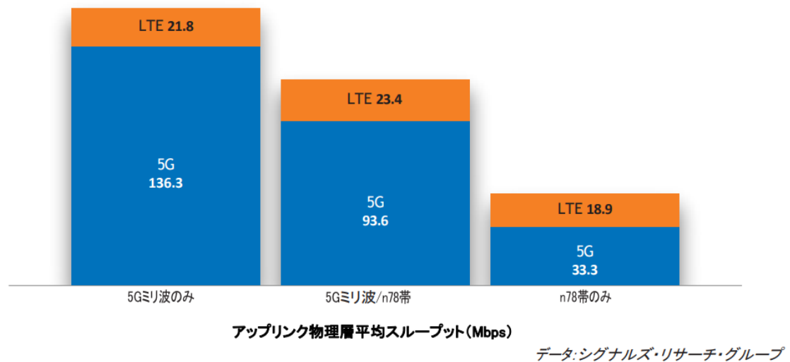
Fig. 5-6 5G millimeter wave uplink throughput mobile measurement outdoors [2]-[3] (English version is available in [3] with registration)
