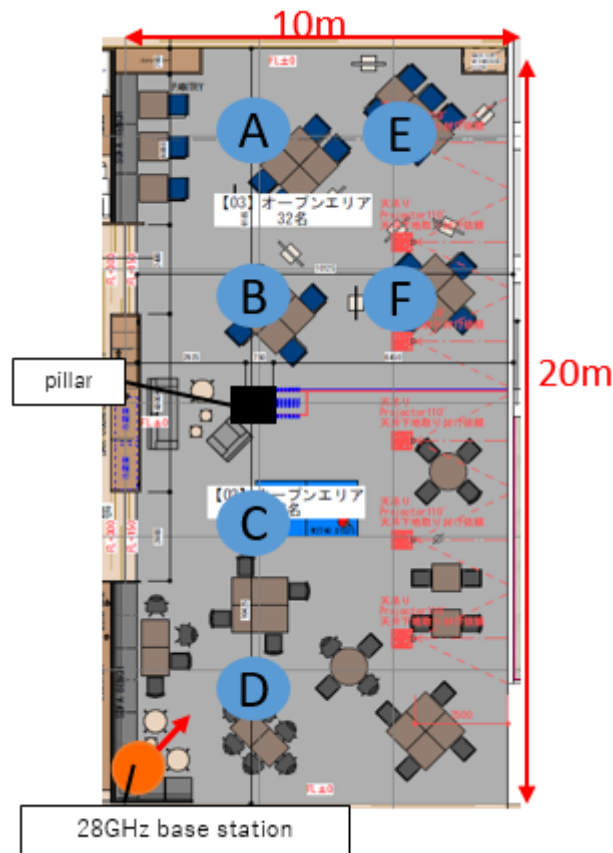
Fig. 5-3 Indoor measurement of 5G mm Wave throughput
