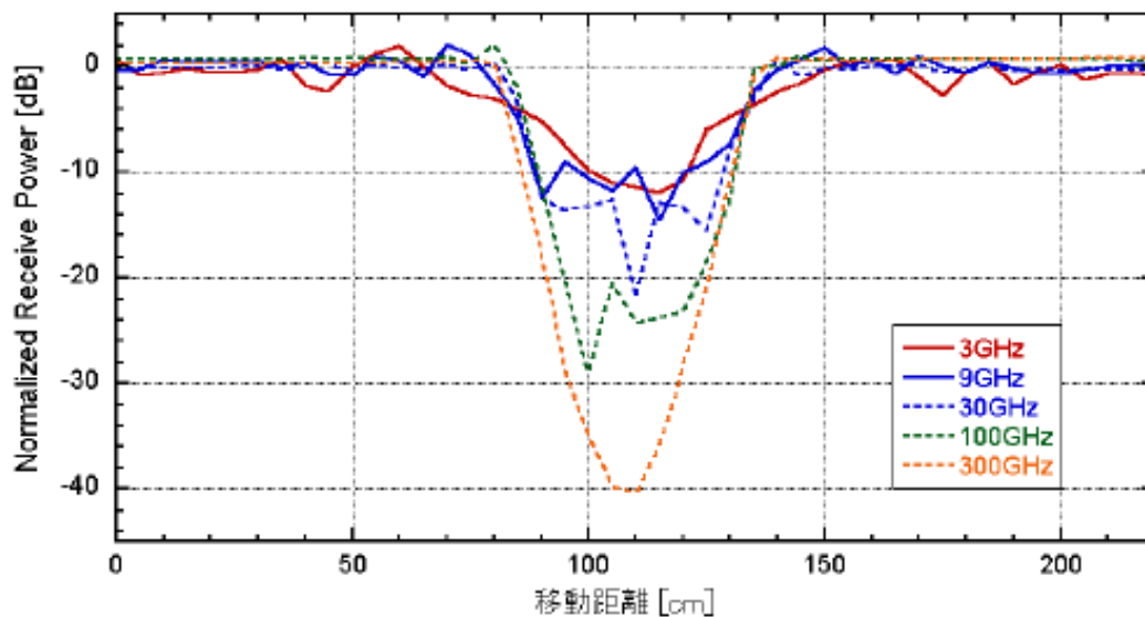
Fig. 3-1 Example of shielding loss measurement results [1]
