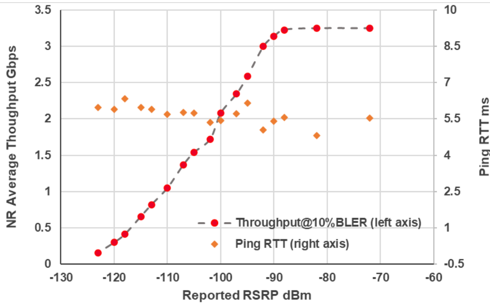
Fig. 5-2 5G millimeter wave throughput and round-trip delay
