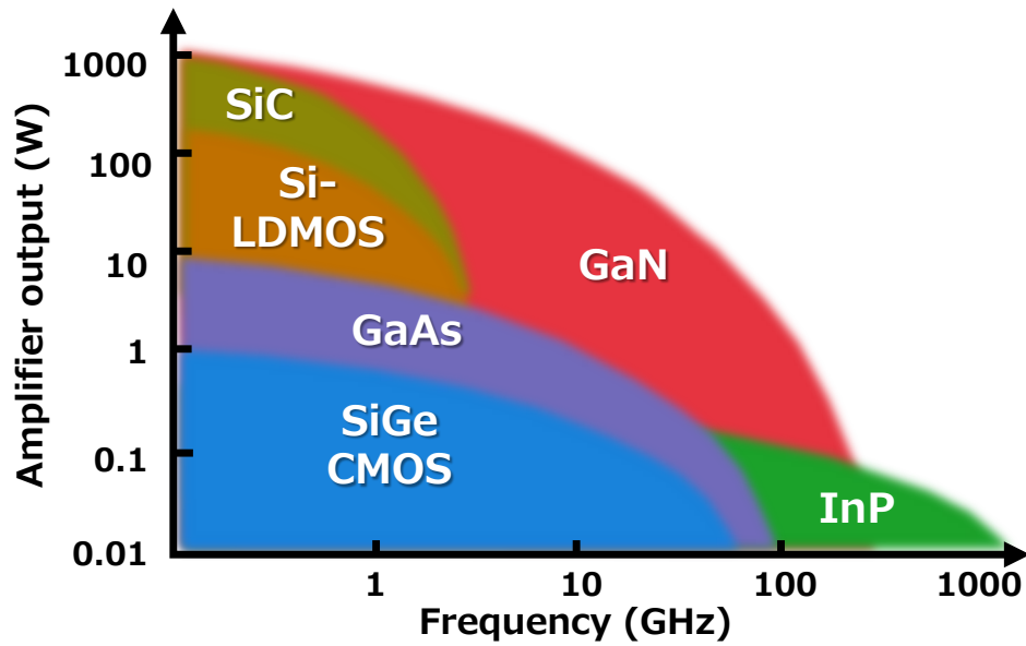
Fig. 4-1 Relationship between frequency and amplifier output
