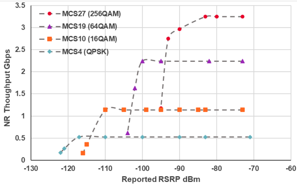
Fig. 5-1 5G millimeter wave throughput
