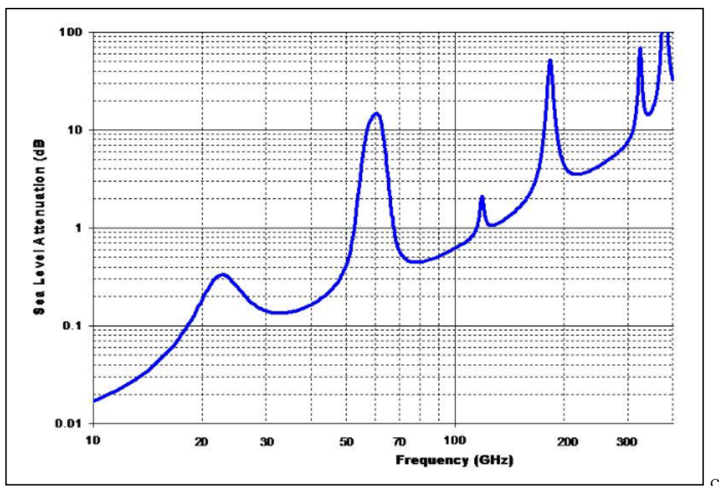
Fig. 3-1 Atmospheric and molecular absorption
