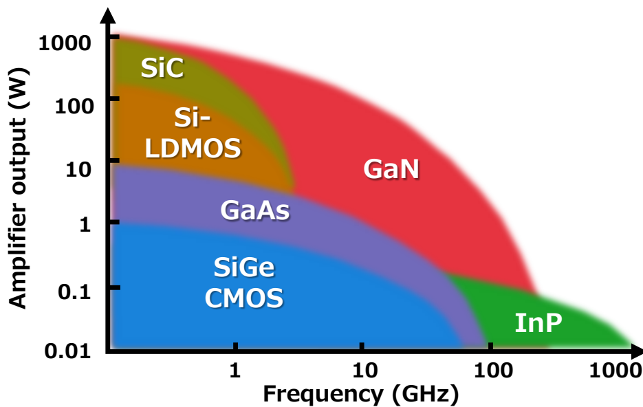
Fig. 4-5 Relationship between frequency and amplifier output
