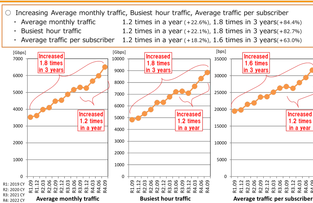
Fig. 1-1 Changes in mobile communication traffic [1]
