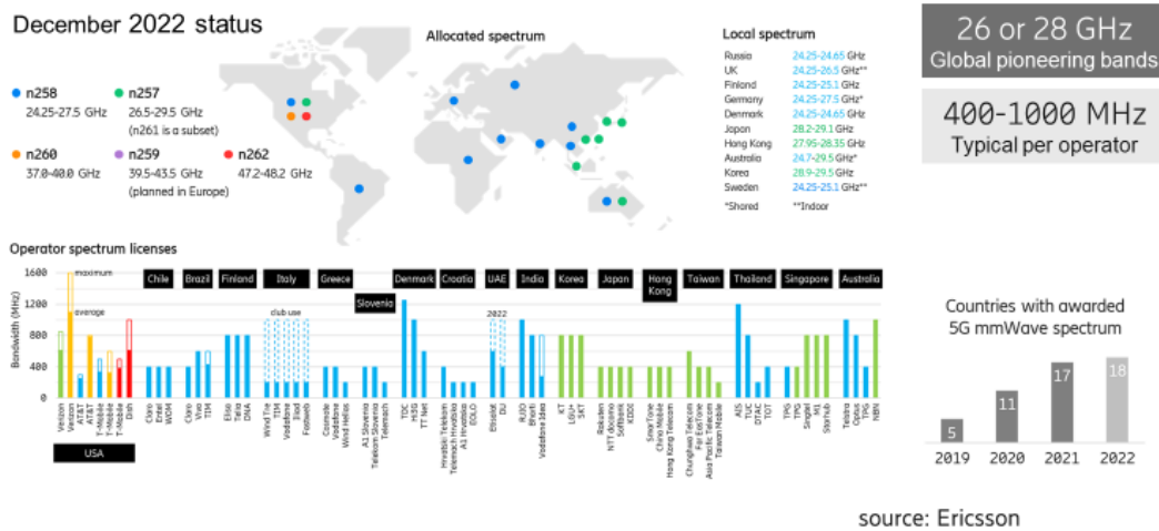
Fig. 2-2 Global millimeter wave spectrum (as of December 2022) [2]
