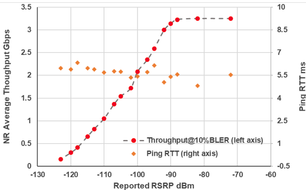
Fig. 5-3 5G millimeter wave throughput and round-trip delay
