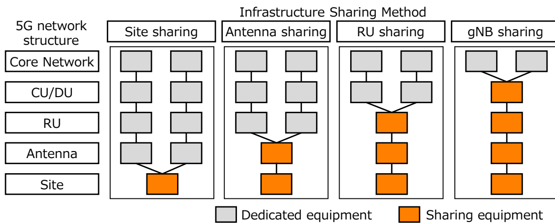
Fig. 4-6 Infrastructure sharing methods
