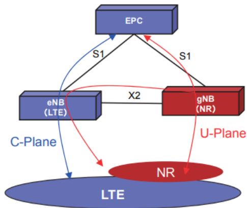
Fig. 4-8 Concept of LTE-NR dual connectivity
