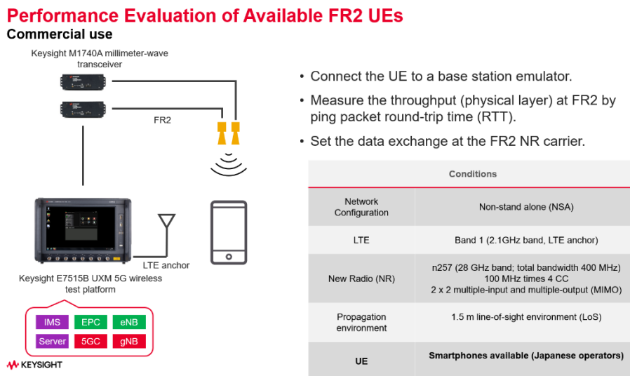
Fig. 5-1 Performance evaluation of commercial terminal (provided by Keysight)
