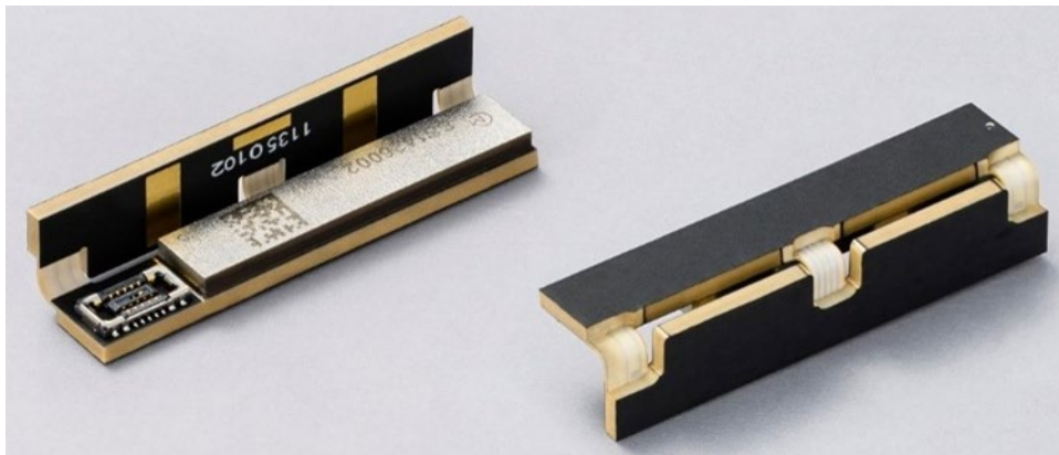
Fig. 9-4 L-shape Antenna Array Integrated Module (by Murata)
