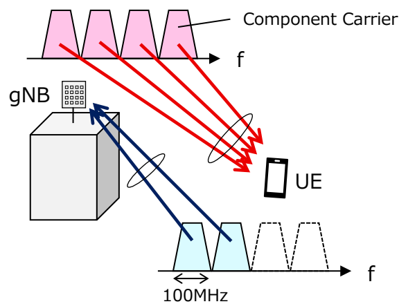
Fig. 4-7 Millimeter wave carrier aggregation (CA)
