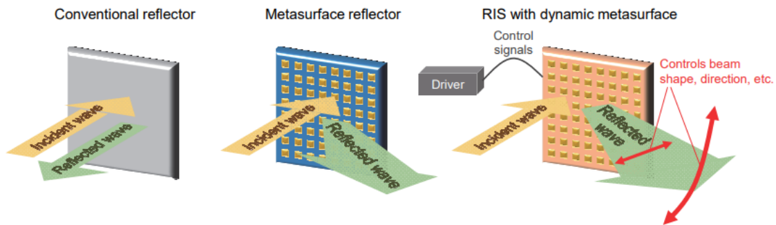
Fig. 4-4 Conceptual diagram of RIS using metasurface technology
